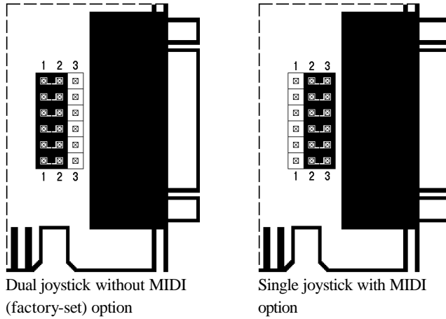
Figure 2. Joystick Jumper Selection
